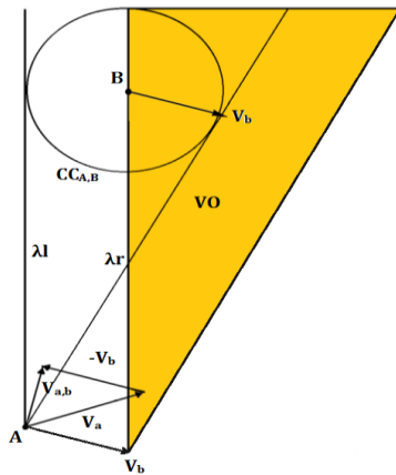
Velocity Obstacles
